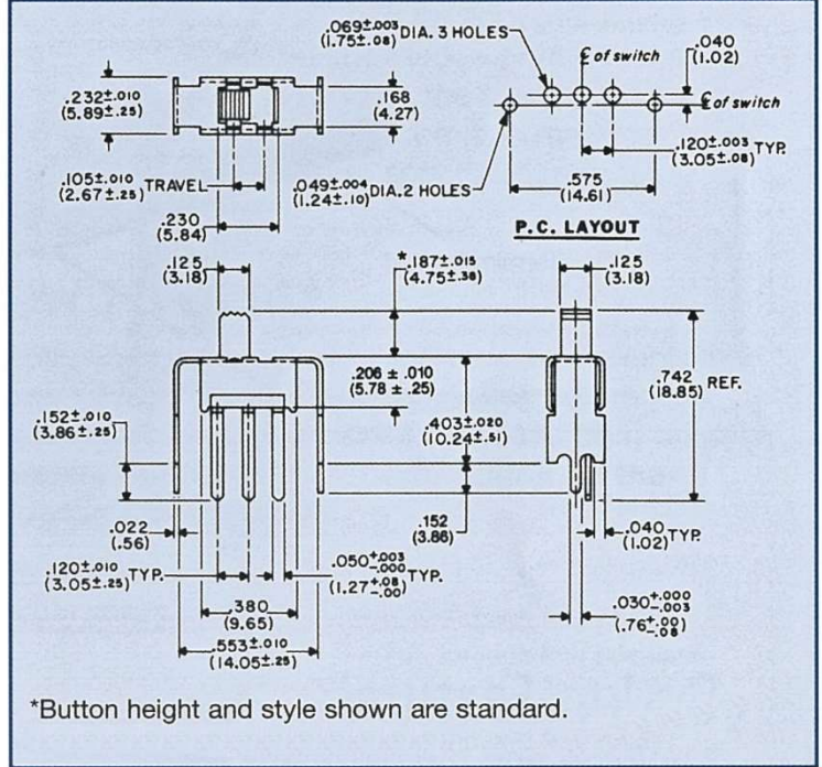
GS-115-PC 0.5 A at 125 Vac/Vdc
