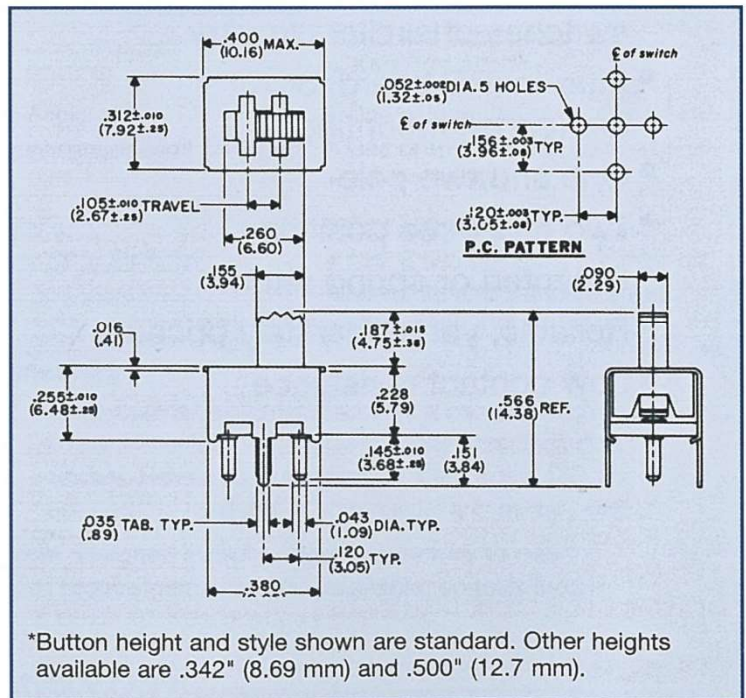
GS-111-PC 0.5 A at 125 Vac/Vdc
