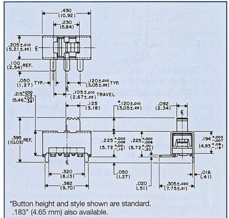
GS-100 0.5 A at 125 Vac/Vdc
