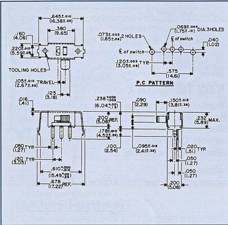
GI-116 0.5 A at 125 Vac/Vdc
