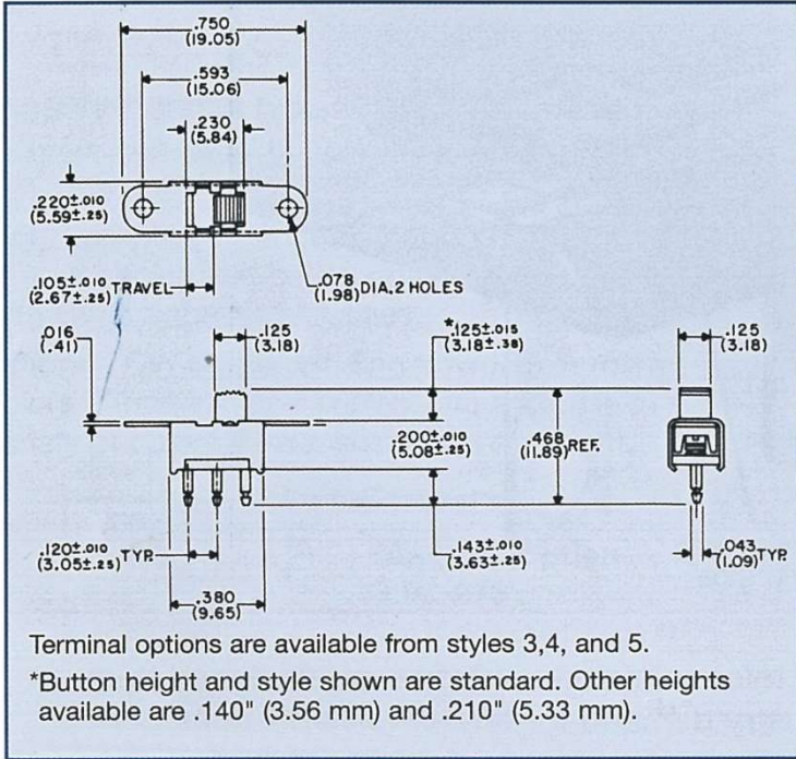
GS-115 0.5 A at 125 Vac/Vdc
