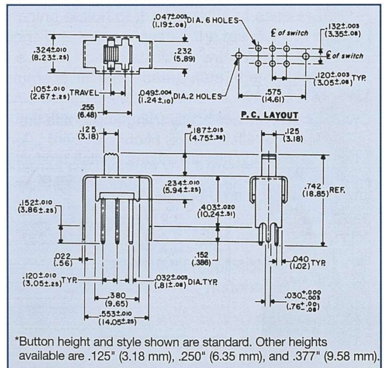
GS-113-PC 0.5 A at 125 Vac/Vdc
